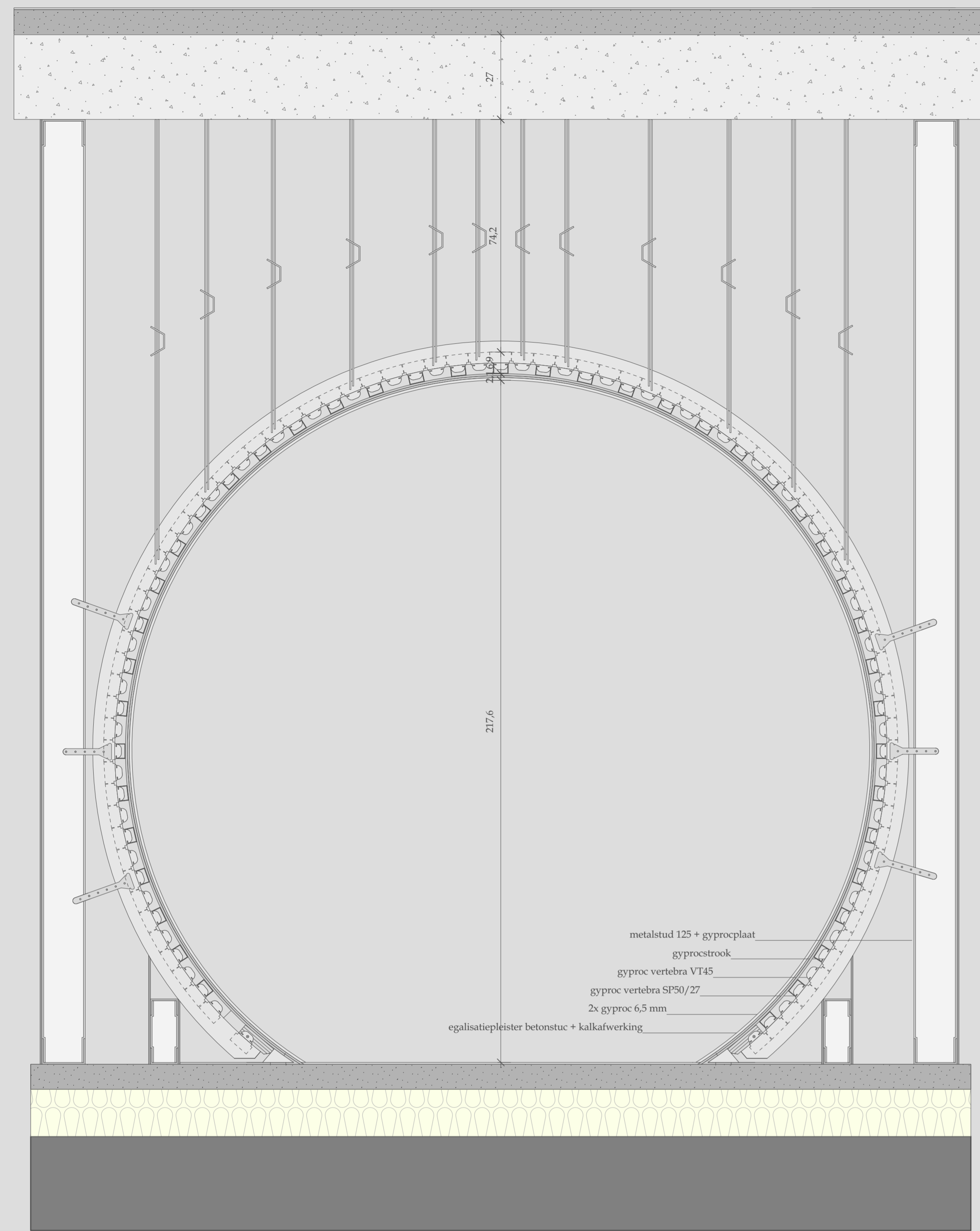
DETAIL BOOG - 1/10
